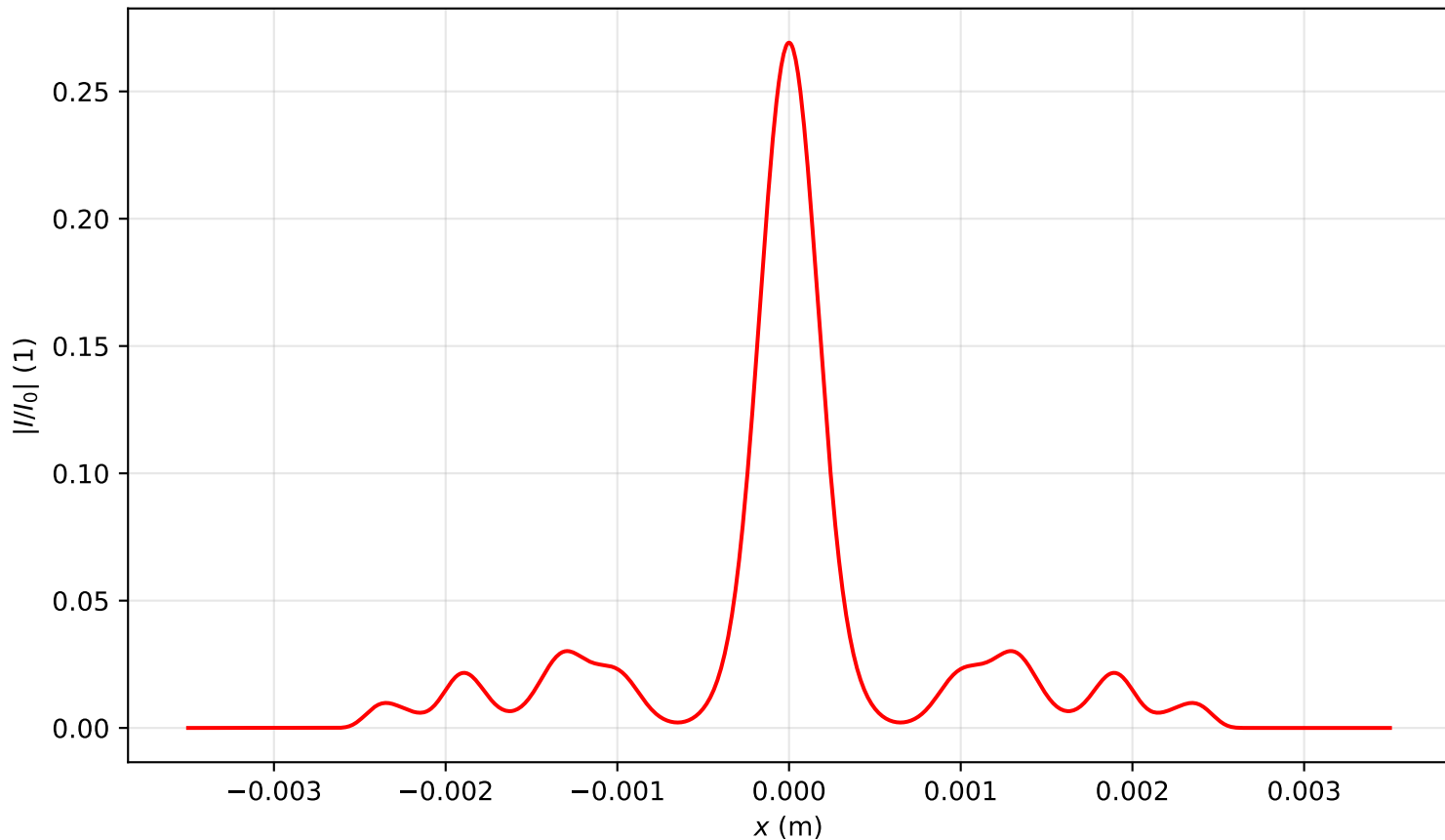
Intensity profile I(x, y = 0, z = 3.582)/I_0 , P_{in}=9.0P_{cr} , artificial time
